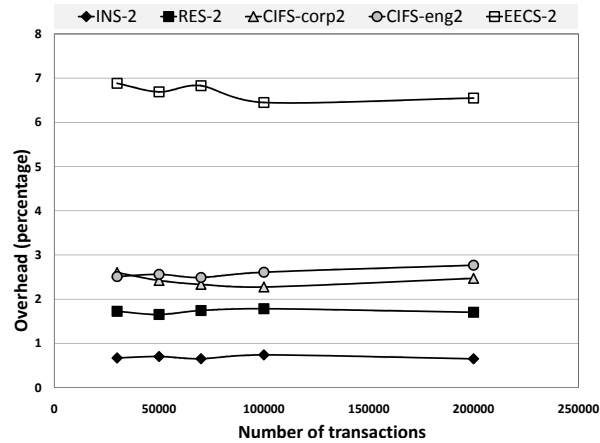
Fig. 9. Overhead for five different workloads ( Config-RD ).
